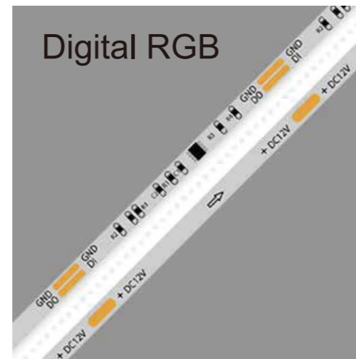
SL-COB-630SM16703
